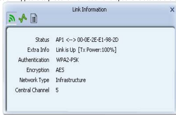
Link information page
