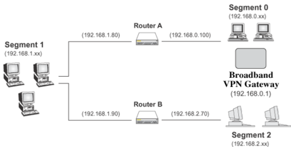
Figure 117: Routing Example
