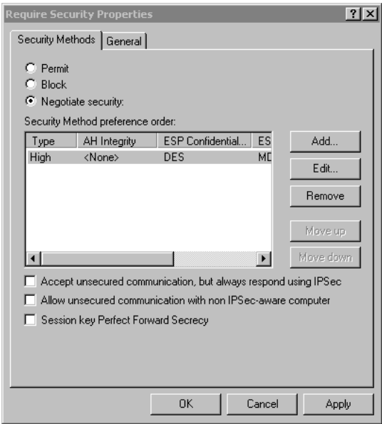
Figure 74: Security Methods
