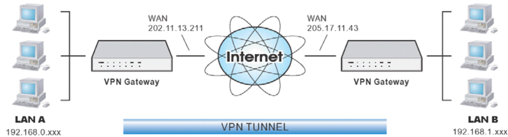
Figure 56: Connecting 2 Broadband VPN Gateways
