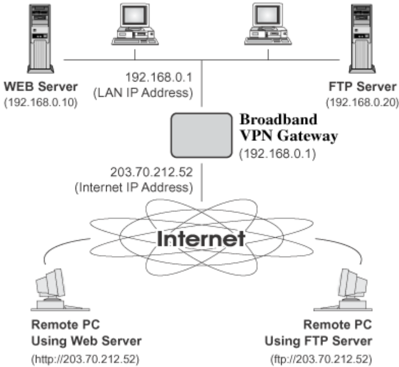
Figure 31: Virtual Servers
