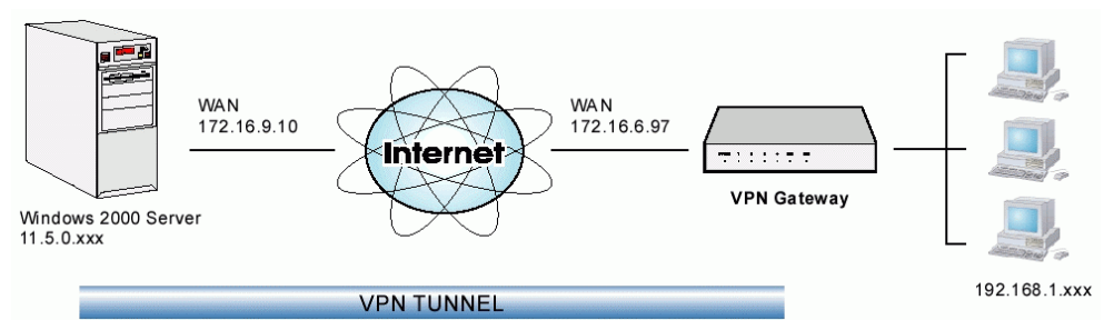
Figure 84: Broadband VPN Gateway to Windows 2000 Server
