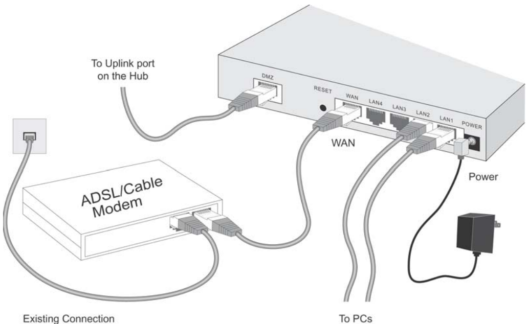
Figure 4: Installation Diagram
