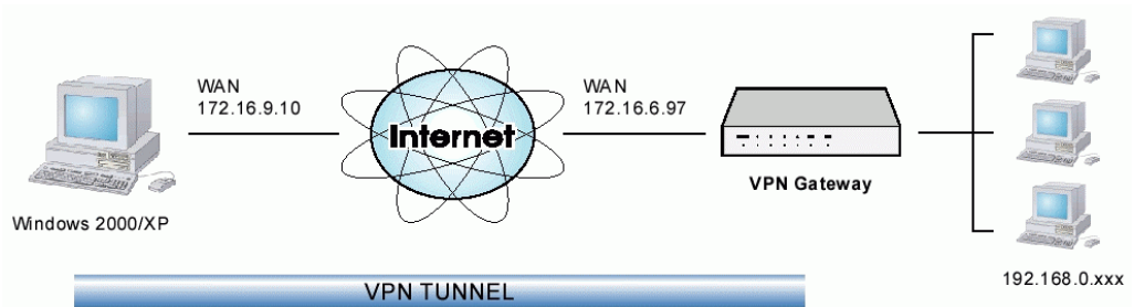
Figure 57: Windows 2000/XP Client to Broadband VPN Gateway
