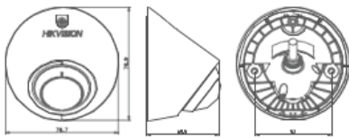
Turret Bracket
