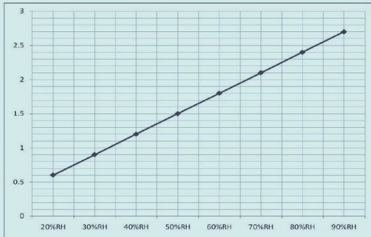
Voltage
